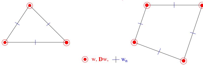
Fig. 10 C^1 VEM, HCT-like
