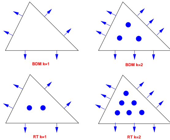
Fig. 7 Face FEM, k=1 and k=2
