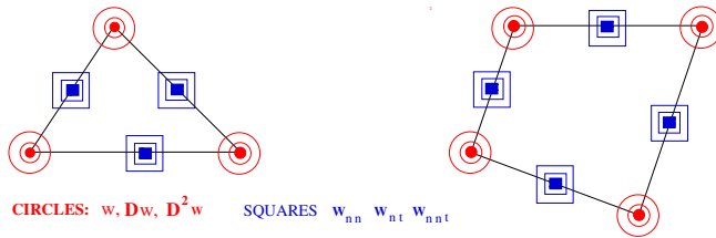
Fig. 14 Examples of C^2 elements
