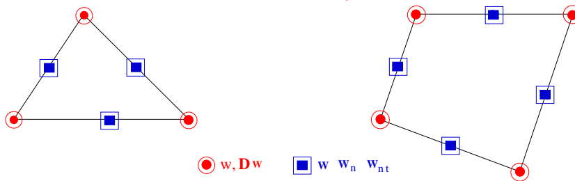
Fig. 11 C^1 VEM, Quartic w and cubic w_{/n}
