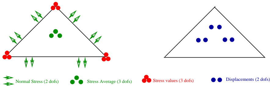
Fig. 20 Hellinger-Reissner Dofs for k = 1 , FEM Arnold-Winther AAW-sym-elast [5]
