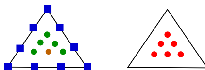
Fig. 16 Dofs for k = 3 , on triangles, for velocities (left) and pressures (right)
