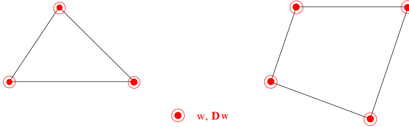
Fig. 9 C^1 VEM, reduced HCT-like
