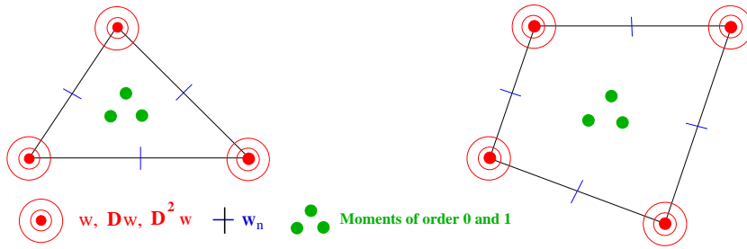
Fig. 12 C^1 VEM, Quintic w and quartic w/n
