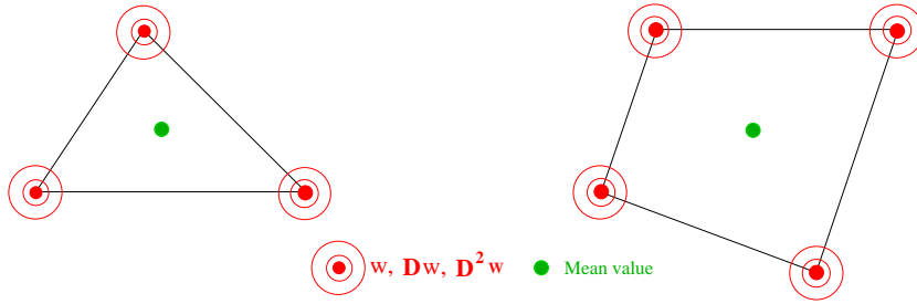
Fig. 13 C^1 VEM, Quintic w and cubic w/n
