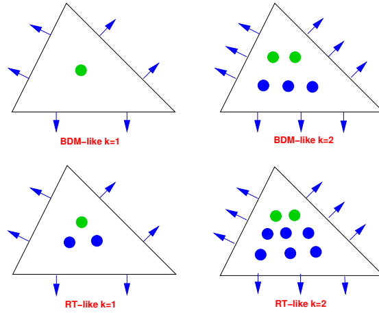
Fig. 8 Face VEM k=1 and k=2
